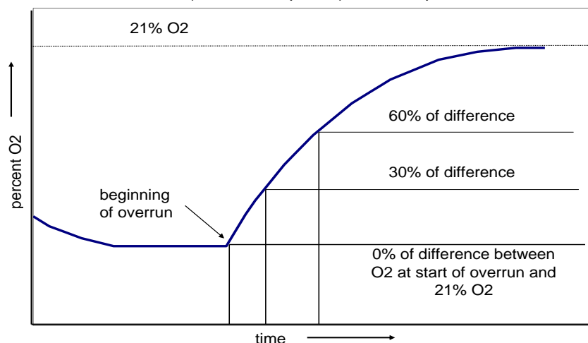
P0133 (O2 slow response) monitor operation
